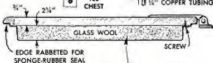
Weather stripping provides a seal for ice-box cover
